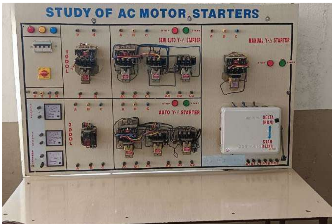
Study of A.C. Motor Starters
