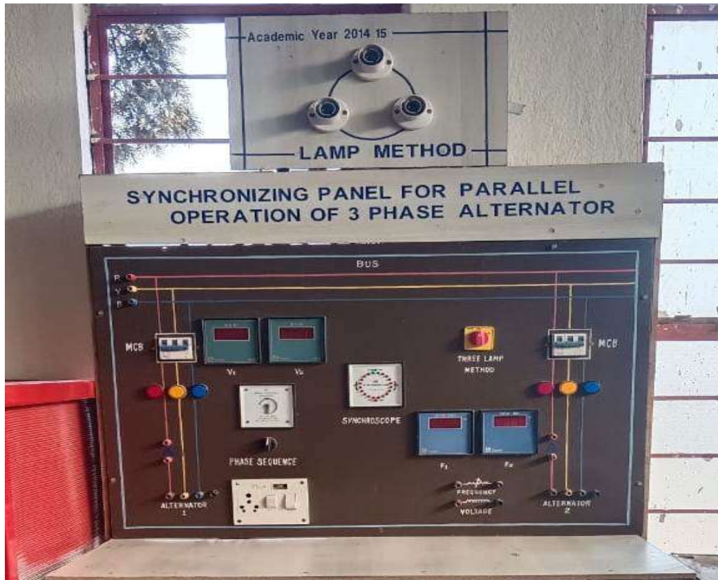
Synchronizing panel for parallel operation of 3 phase alternator
